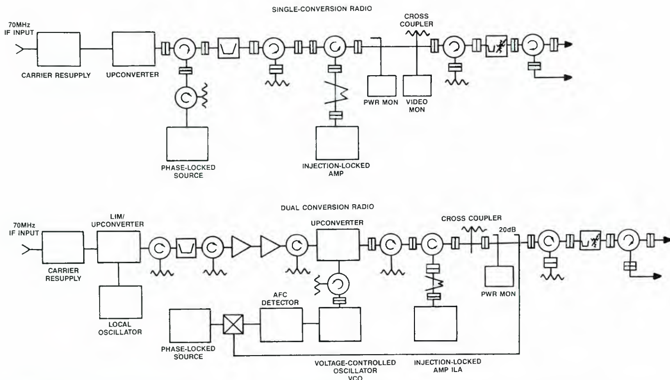
Figure 1. The dual-conversion radio mixes the IF twice, once to create a high IF at 1,470MHz and again to obtain the 7GHz output RF frequency. The dual-conversion technique was kept for better frequency selectivity and frequency rejection.
