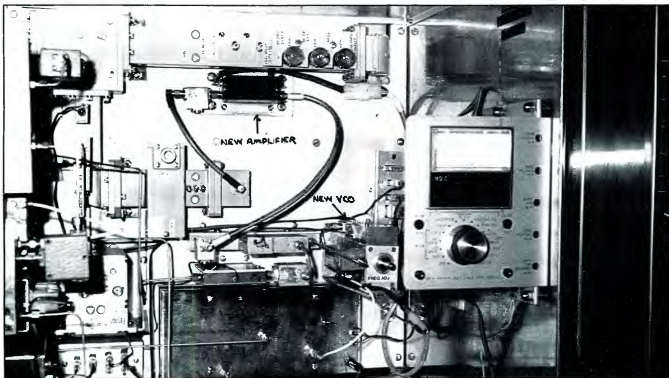
The replacement amplifier and VCO occupy but a small portion of the originally needed space. Because the components draw so little current, no power-supply changes are needed.
