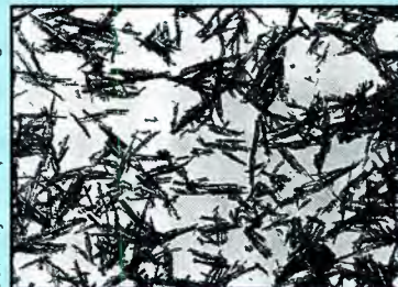
Photomicrograph of metal particles used in the manufacture of metal-particle tape, at a magnification of 70,000 times.
