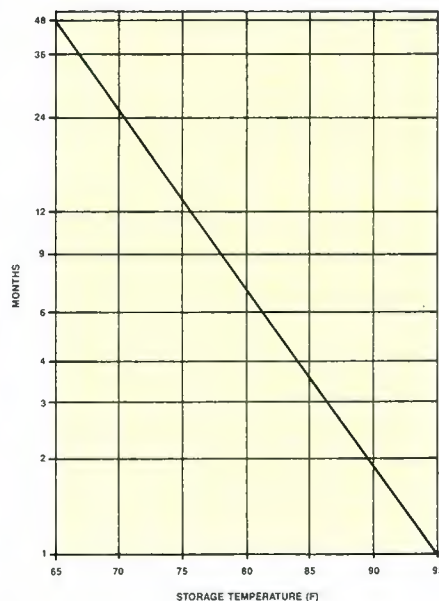
Figure 2. Estimated rewind interval for archived tapes as a function of temperature. Other factors may dictate more frequent rewinding.
