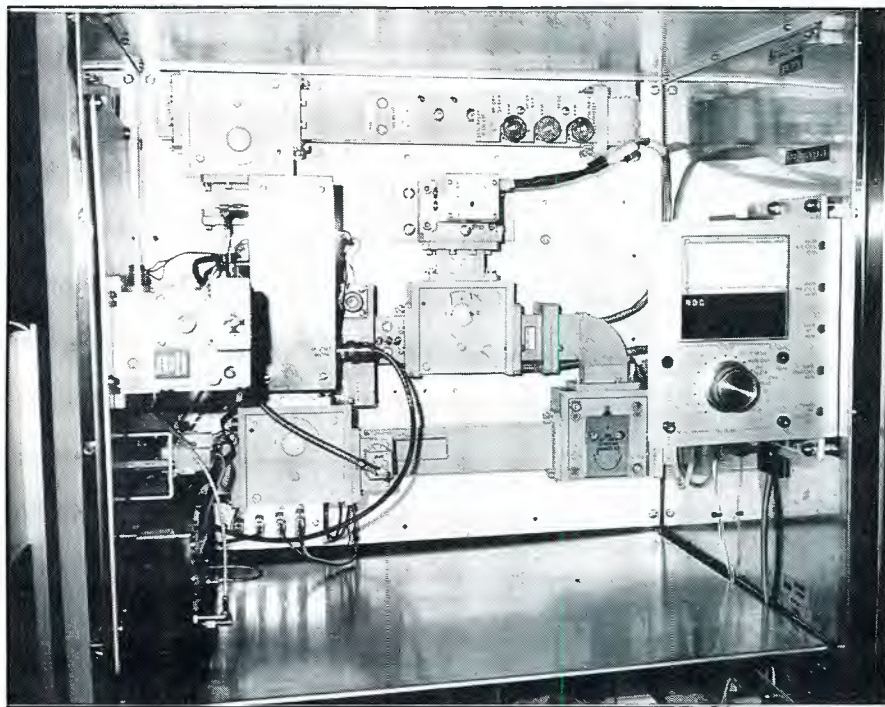
The new ILA, upconverter and phase source in this single-conversion prototype replace all the mixers, amplifiers, VCO and AFC circuitry associated with the dual-conversion design.
